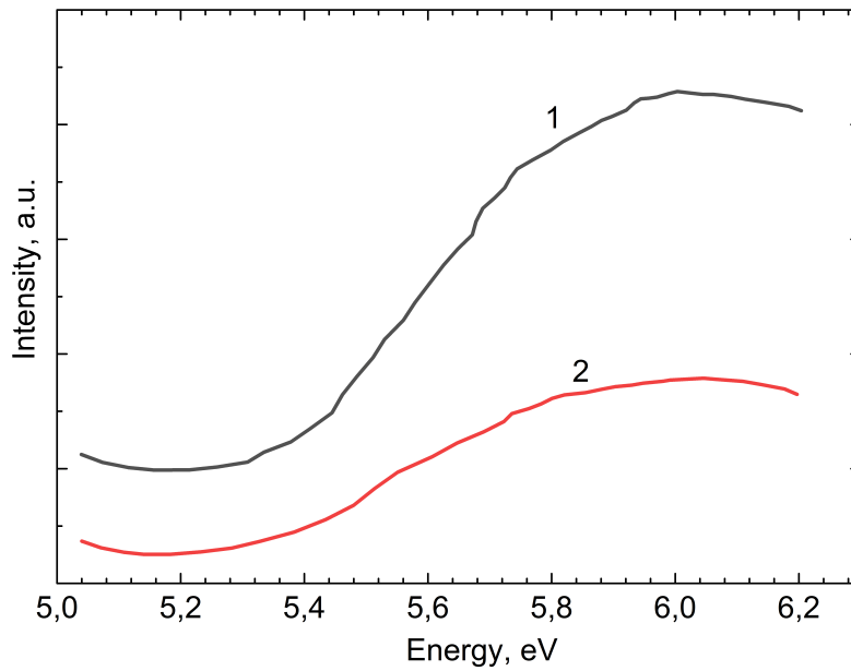
Figure 3. Excitation spectrum of 2.7 eV emission at: 1) 15 K; 2) 300 K.
