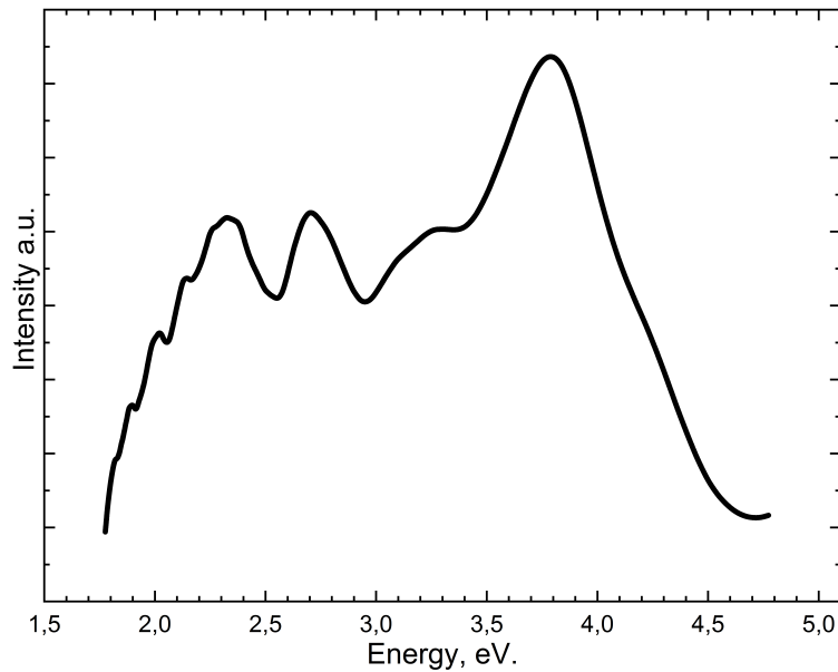
Figure 1. Luminescence of powder \text{SrSO}_4 upon excitation by photons with an energy of 6.5 eV at 300 K.
