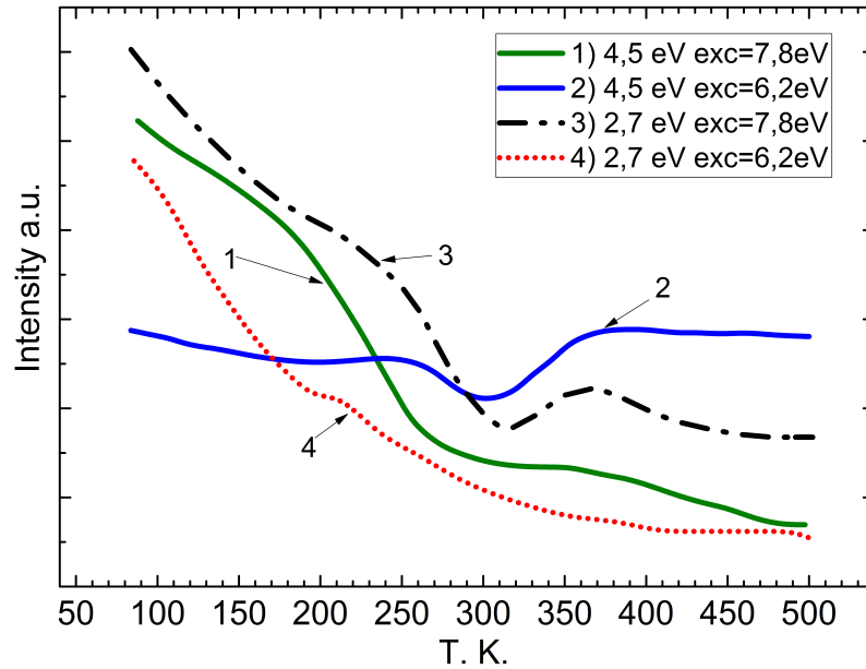
Figure 6. Temperature dependence of luminescence for emission: 4.5 eV upon excitation 1) 7.8 eV, 2) 6.2 eV; 2.7 eV upon excitation 3) 7.8 eV, 6.2 eV.
