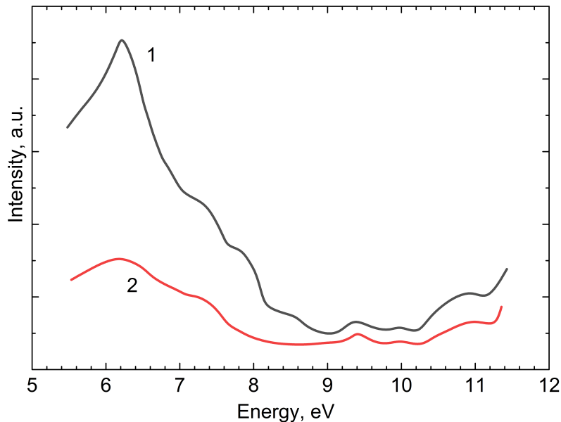
Figure 4. Excitation spectrum for the 2.7 eV emission at: 1) 80 K; 2) 300 K.
