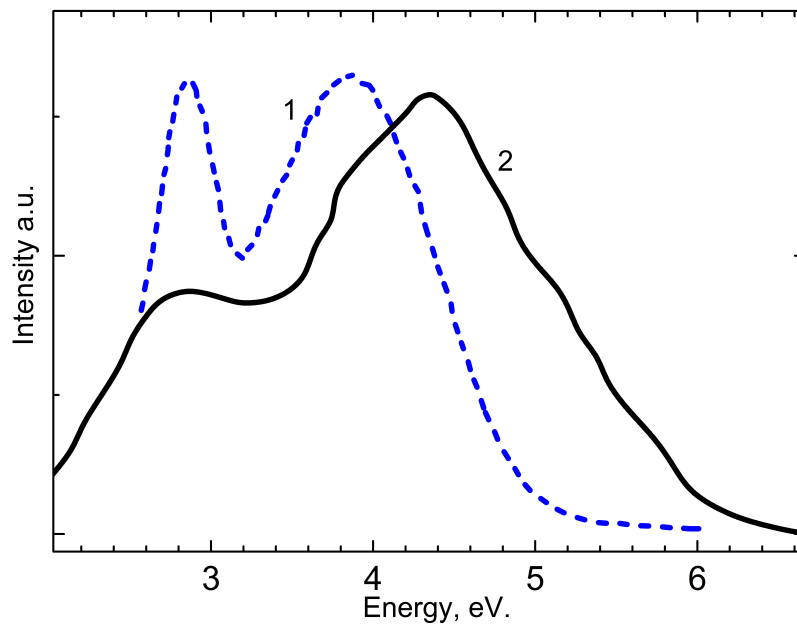
Figure 2. Luminescence of \text{SrSO}_4 upon excitation by photons with energies: 1) 8 eV; 2) 10-12 eV; at 15 K.
