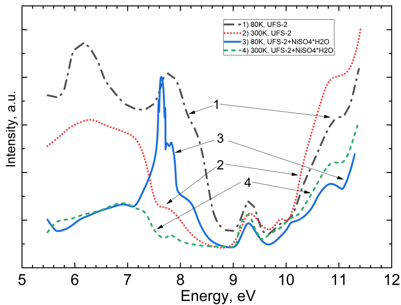
Figure 5. Excitation spectrum of the 4.5 eV emission band with filter UFS-2: 1) 80 K; 2) 300 K; with filter UFS-2+ NiSO 4 : 3) 80 K; 4) 300 K.
